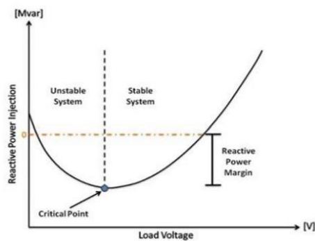
Figure 2 Q-V Curve (Reactive Power vs. Voltage)
