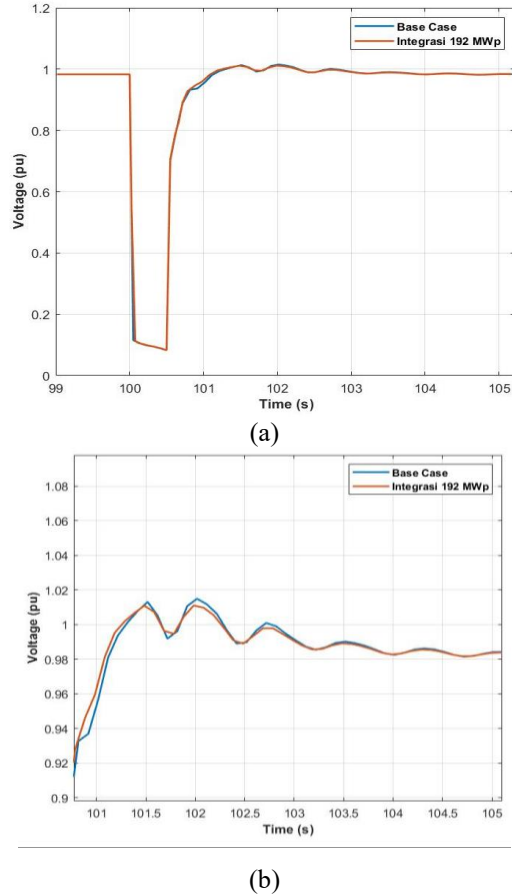
Figure 12 Dynamic Voltage Response Graph at Bus 11: (a) Full Graph Condition (b) Overshoot
