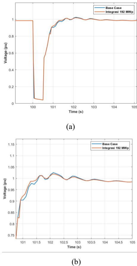
Figure 10 Dynamic Voltage Response Graph at Bus 25: (a) Full Graph Condition (b) Overshoot
