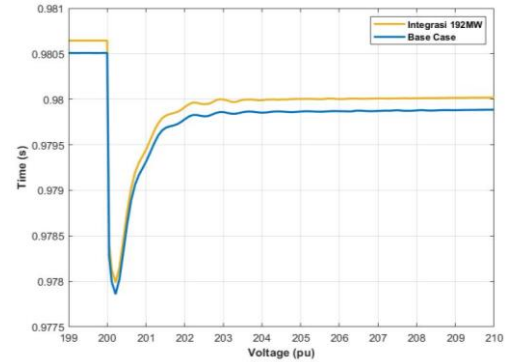
Figure 13 Dynamic Voltage Response Graph at Bus 9 during Load Increase
