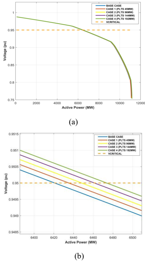
Figure 8 P-V Curve Results at Busbar 9 Cibatu: (a) Nose Curve Condition Reached, (b) Critical Voltage Condition
