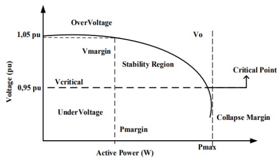
Figure 1 P-V Curve Graph (Active Power vs. Voltage)
