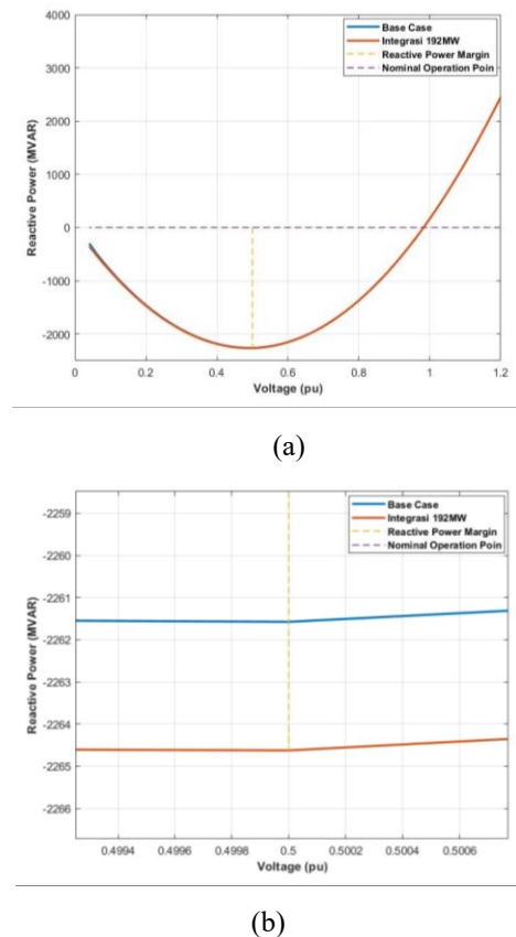
Figure 9 Q-V Curve Results at Busbar 10 Cirata: (a) Full Curve Condition (b) Reactive Power Margin
