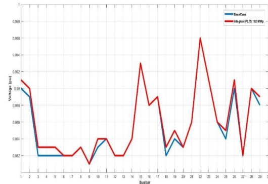
Figure 5 Load Flow Results on Voltage Profile
