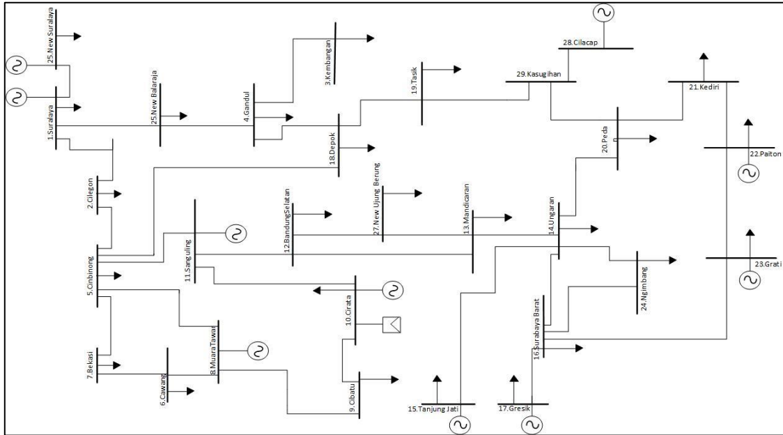
Figure 4 Single Line Diagram of the Java-Bali 500 kV Transmission System
