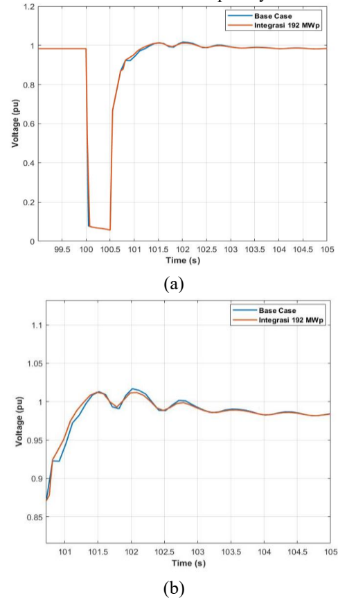
Figure 11 Dynamic Voltage Response Graph at Bus 8: (a) Full Graph Condition (b) Overshoot
