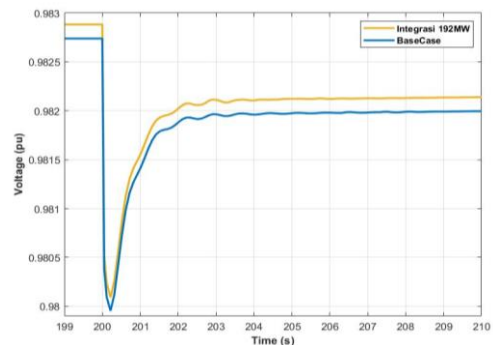
Figure 14 Dynamic Voltage Response Graph at Bus 12 during Load Increase
