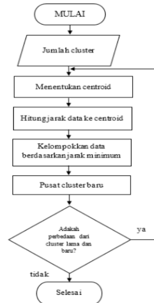
Gambar 4. Flowchart metode
