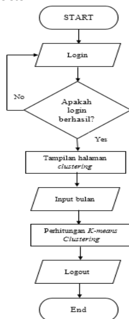
Gambar 3. Flowchart Sistem
