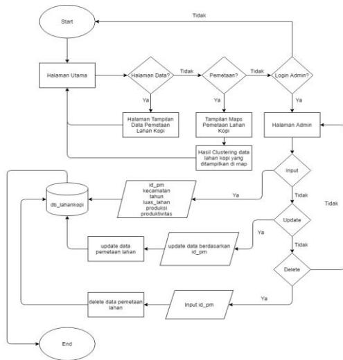
Gambar 2. Flowchart Sistem
