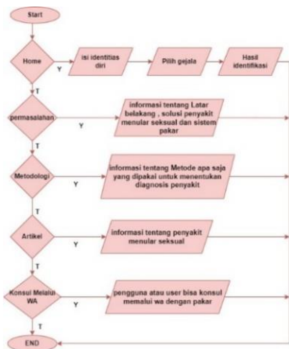
Gambar 3. Flowchart user
