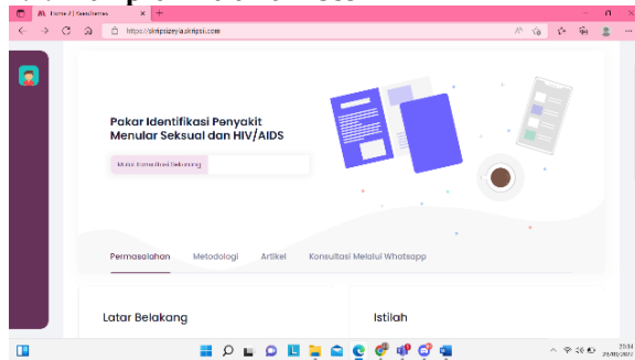
Gambar 7. Halaman User
