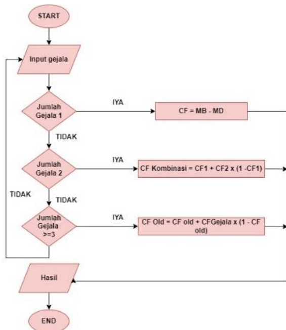
Gambar 5. Flowchart Metode
