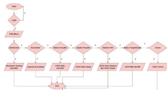
Gambar 4. Flowchart sistem
