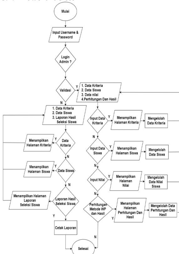
Gambar 2. Flowchart Sistem
