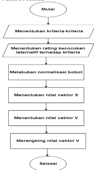
Gambar 5. Flowchart Metode
