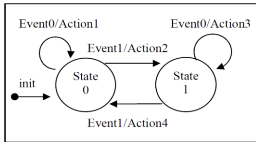
Gambar 1. Diagram FSM
