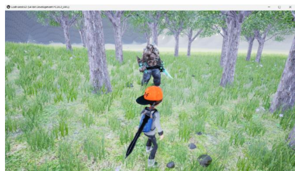
Gambar 9. Level 2
