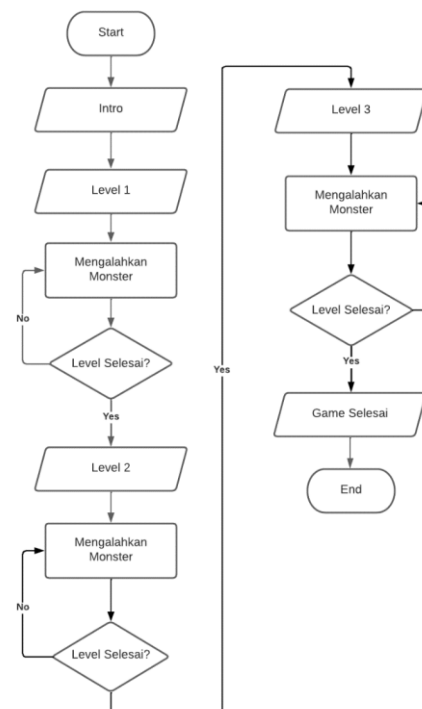
Gambar 2. Flowchart Permainan
