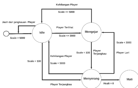
Gambar 4. Diagram FSM
