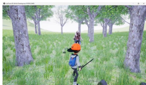
Gambar 8. Level 1
