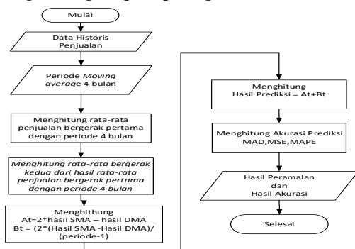
Gambar 1. Flowchart metode
