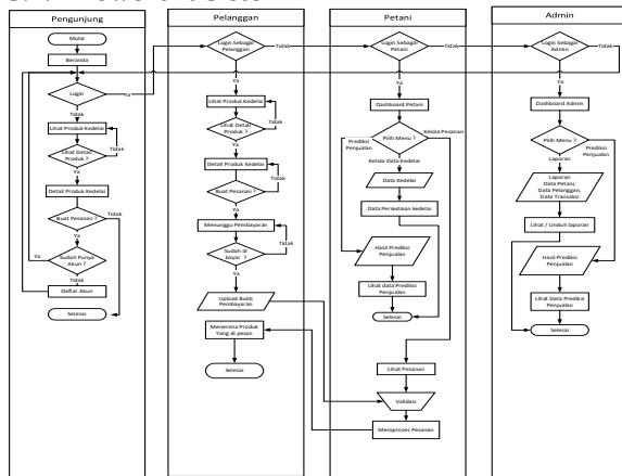
Gambar 5. Flowchart Sistem
