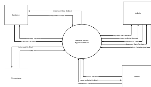
Gambar 3. DFD Level 0
