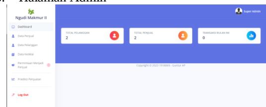
Gambar 8. Halaman Admin
