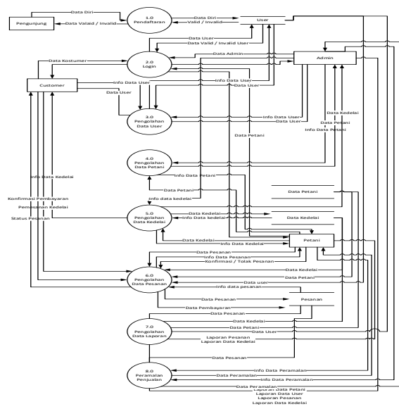
Gambar 4. DFD Level 1
