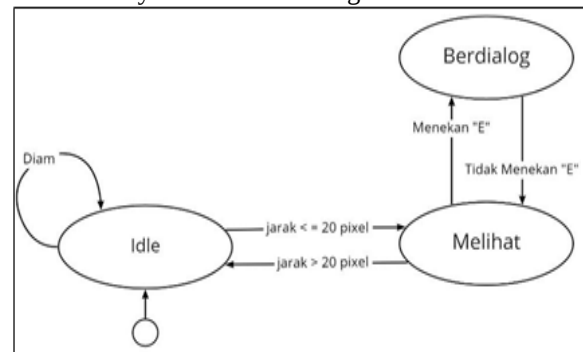
Gambar 2 Diagram Finite State Machine
