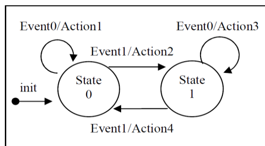
Gambar 1 .Diagram Finite State Machine
