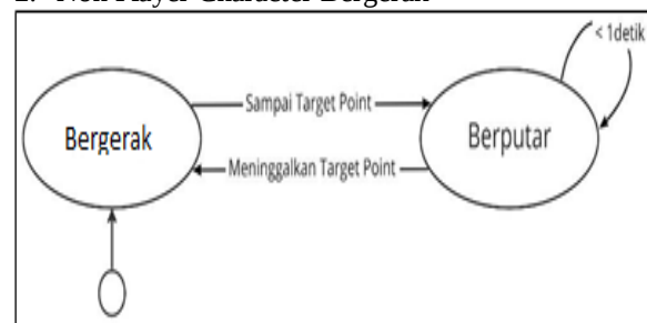
Gambar 3 Diagram Finite State Machine Bergerak
