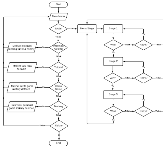
Gambar 2. Flowchart game
