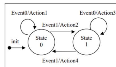
Gambar 1. Diagram finite state machine [10]
