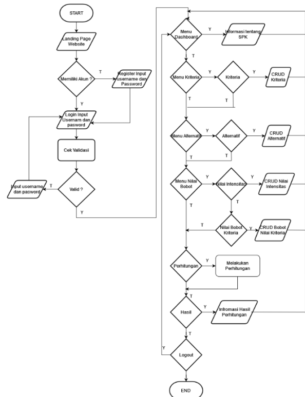
Gambar 3. Flowchart sistem
