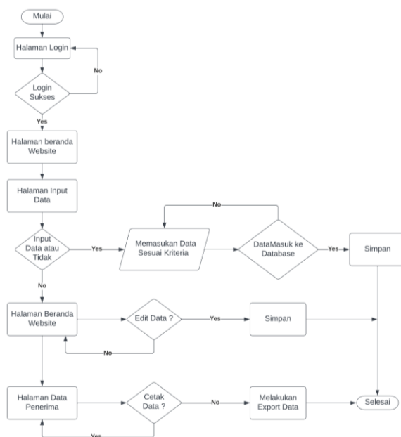
Gambar 5. Flowchart sistem
