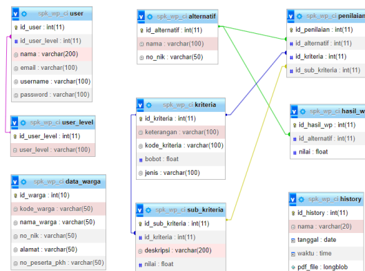
Gambar 3. Class diagram
