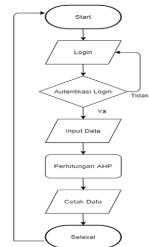
Gambar 1 Flowchart sistem
