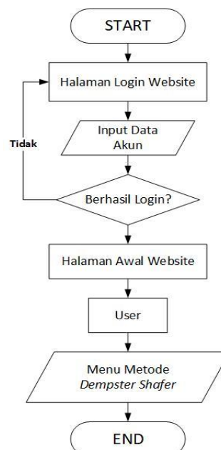
Gambar 5. Flowchart Admin
