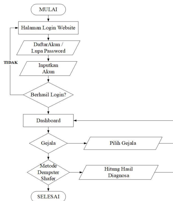
Gambar 6. Flowchart User
