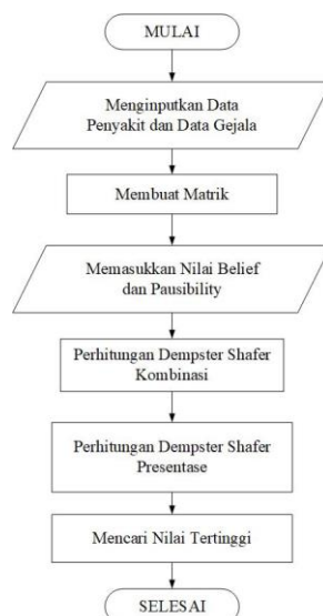
Gambar 7. Flowchat Metode
