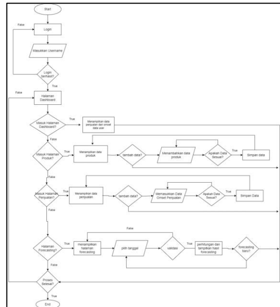
Gambar 4 Flowchart Alur Sistem
