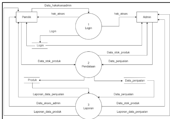
Gambar 2 DFD Level 1
