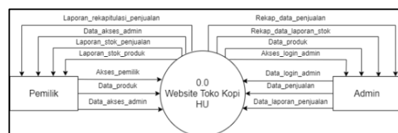
Gambar 1 DFD Level 0
