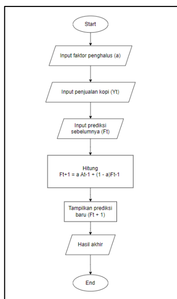
Gambar 3 Flowchart Metode
