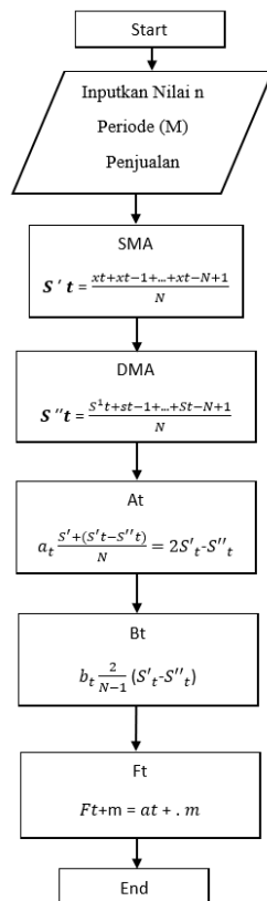
Gambar 3. Flowchart Metode
