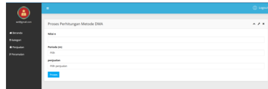
Gambar 4. Halaman Peramalan
