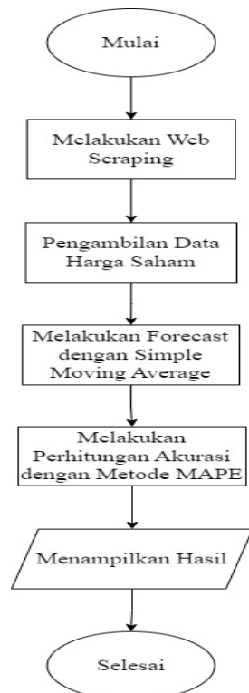
Gambar 3 Flowchart sistem
