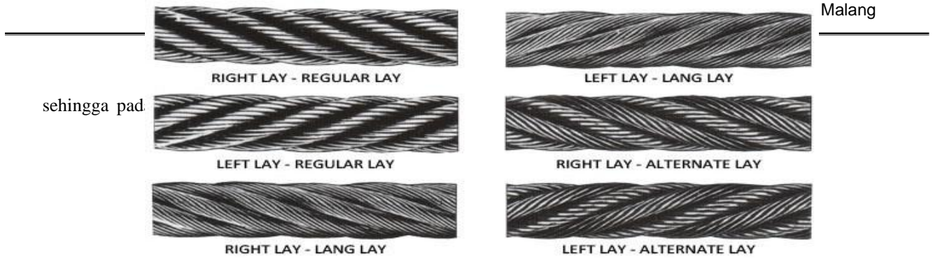
Gambar 2.5 Kabel Wire Rope
