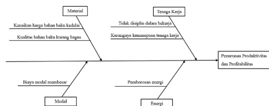
Gambar 3. Diagram Fishbone
