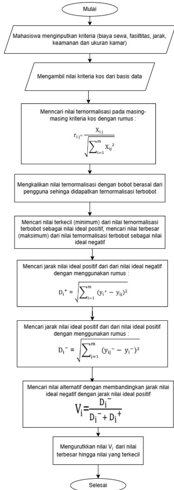
Gambar 3. Flowchart Metode
