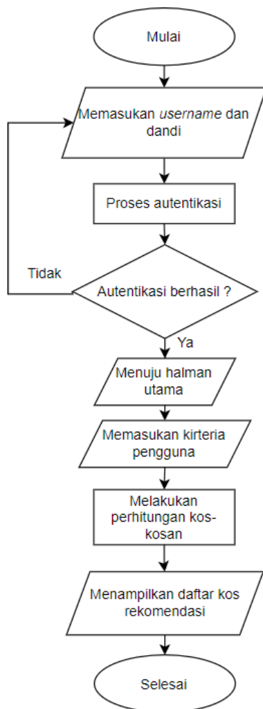
Gambar 2. Flowchart Sistem
