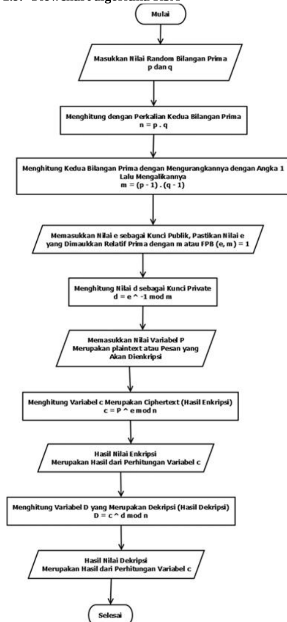
Gambar 1. Flowchart RSA
