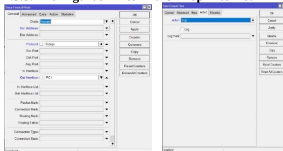
Gambar 13. Konfigurasi Filter Rule Drop
