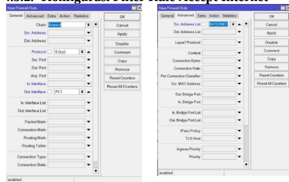
Gambar 12. Konfigurasi filter rule
