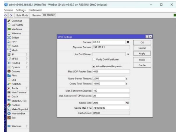
Gambar 8. Menu setting dns server
