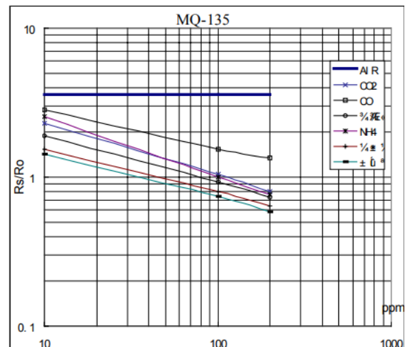
Gambar 8. Datasheet MQ-135
