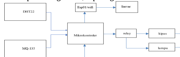
Gambar 1. Diagram Sistem
