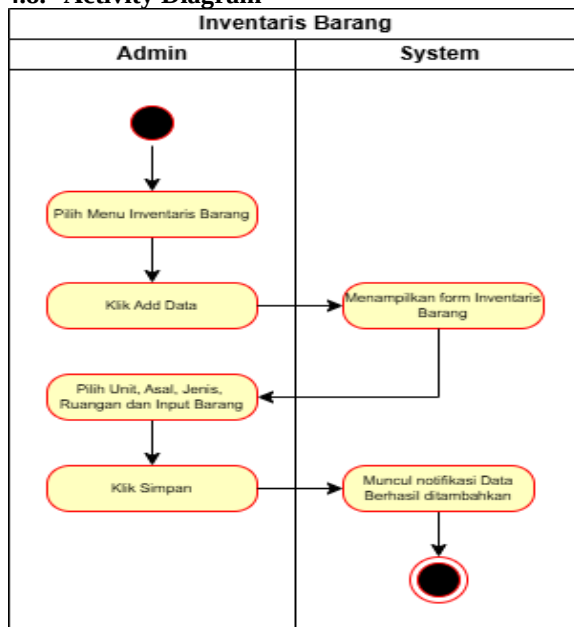
Gambar 6. Activity diagram inventaris barang
