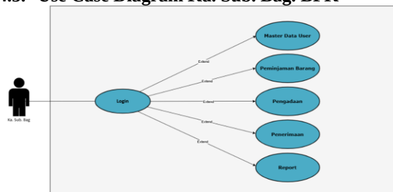
Gambar 4. Use case diagram ka. sub. bag. BPK
