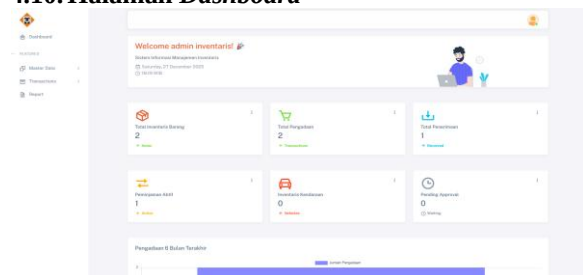
Gambar 9. Halaman dashboard
