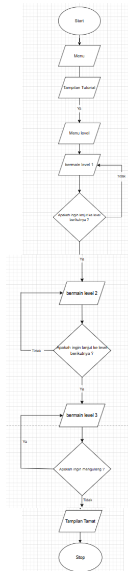
Gambar 2. Flowchart game
