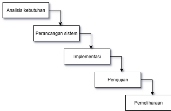
Gambar 1. Diagram Waterfall
