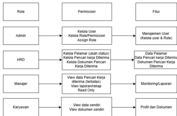
Gambar 8. Diagram RBAC
