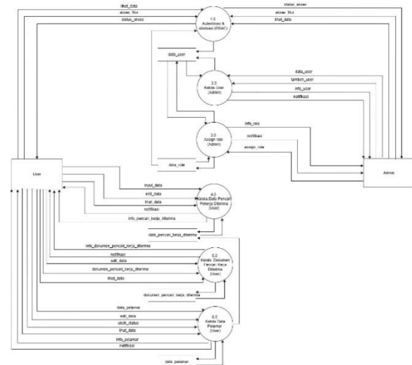
Gambar 5. DFD level 1
