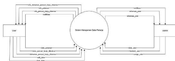
Gambar 4. DFD level 0
