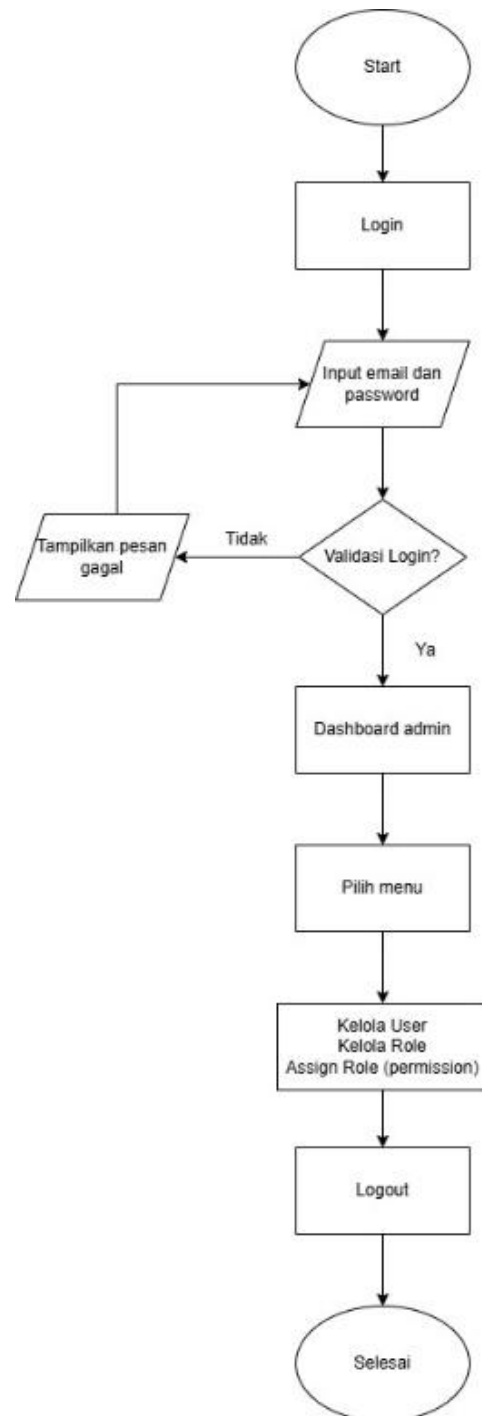
Gambar 2. Flowchart admin
