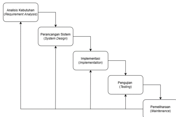
Gambar 1. Diagram waterfall
