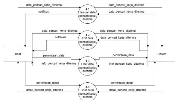
Gambar 6. DFD level 2
