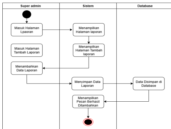
Gambar 6. Diagram Activity Super admin Tambah Data Laporan
