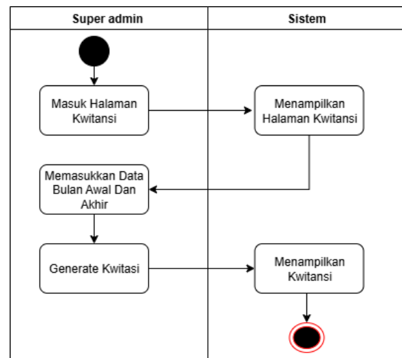
Gambar 8. Diagram Activity Super admin Generate Kwitansi
