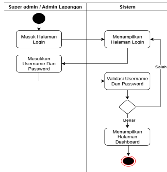
Gambar 3. Diagram Activity Login Super admin & Admin Lapangan
