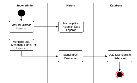
Gambar 7. Diagram Activity Super admin Update Dan Hapus Data Laporan
