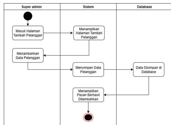
Gambar 4. Diagram Activity Super admin Tambah Data Pelanggan
