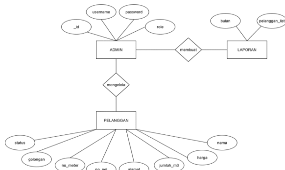
Gambar 10. Entity Relationship Diagram (ERD) Sistem Informasi PDAM Tirta Wening
