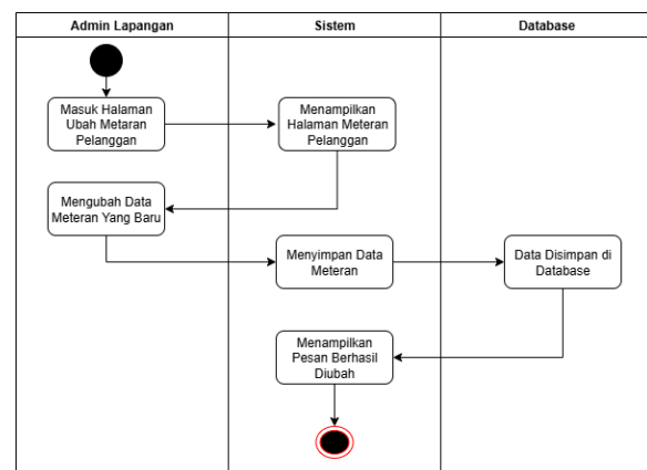
Gambar 9. Diagram Activity Admin Lapangan Ubah Data Meteran Baru
