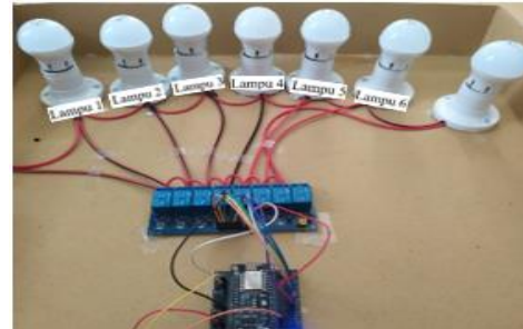
Gambar 9. Pengujian lampu led
