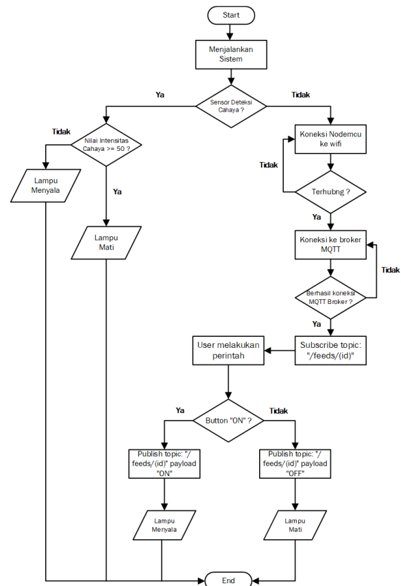
Gambar 4. Flowchart sistem
