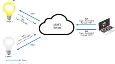
Gambar 11. Proses alur controlling lampu mqtt
