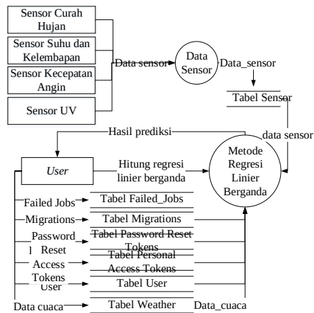
Gambar 7. DFD level 1
