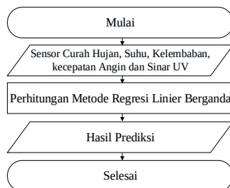
Gambar 3. Flowchart sistem
