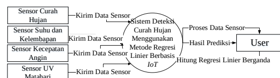
Gambar 6. DFD level 0
