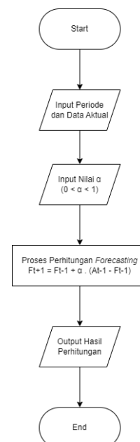
Gambar 2. Flowchart Metode
