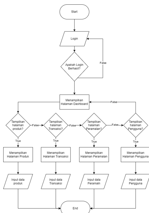
Gambar 4. Flowchart Admin
