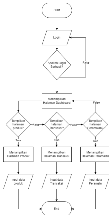
Gambar 3. Flowchart Sistem
