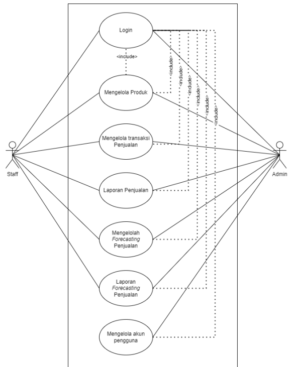
Gambar 1. Usecase Diagram
