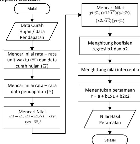
Gambar 2 Flowchart Metode Least Square
