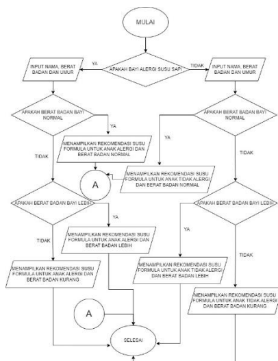
Gambar 3. Flowchart Sistem
