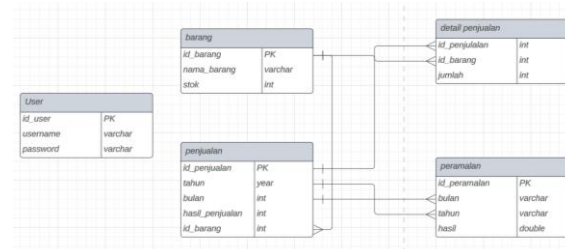
Gambar 3 Diagram Class
