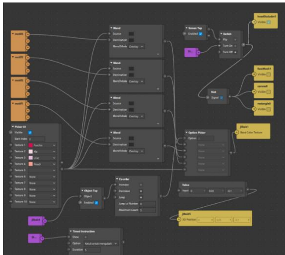
Gambar 8. Patch editor
