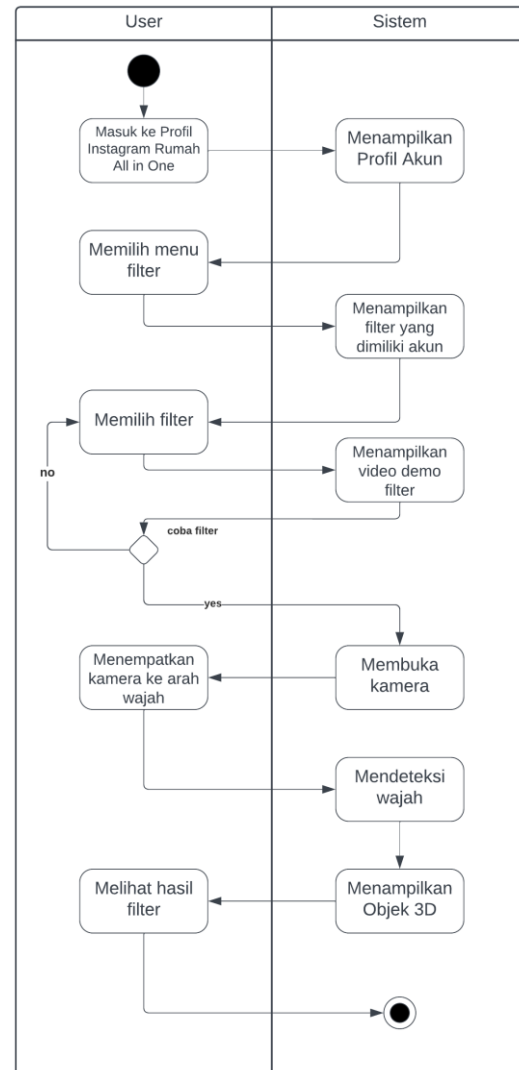
Gambar 2. Activity Diagram
