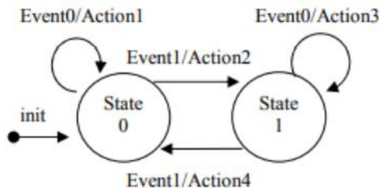
Gambar 1. Diagram Finite State Machine [12]
