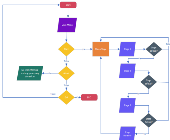
Gambar 2. Flowchart Game
