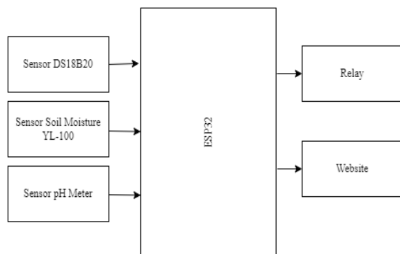
Gambar 8. Diagram Blok
