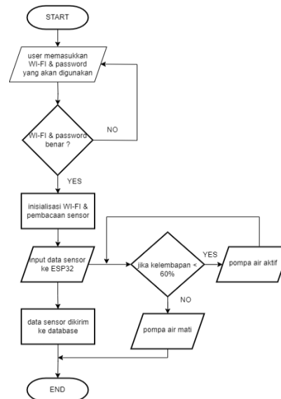
Gambar 9. Flowchart Smart Farming
