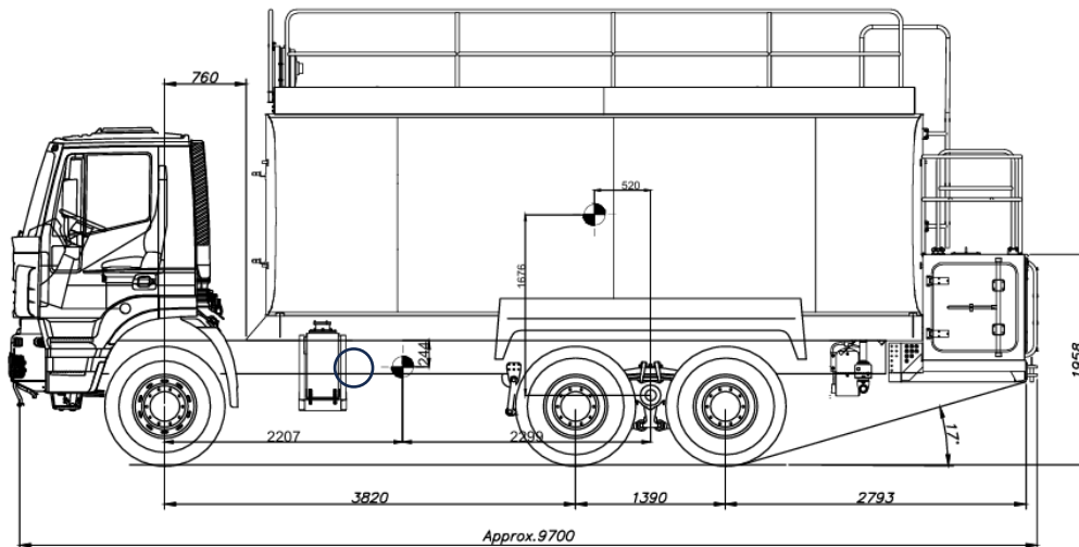
Gambar 1 COG Iveco Trakker AD380T44WH 6x6 fuel truck 25kl
