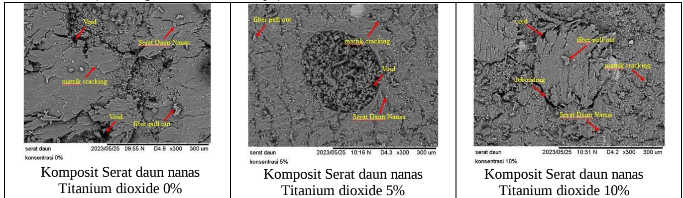
Gambar 3. Hasil Pengujian Sem ( scanning electron microscope )
