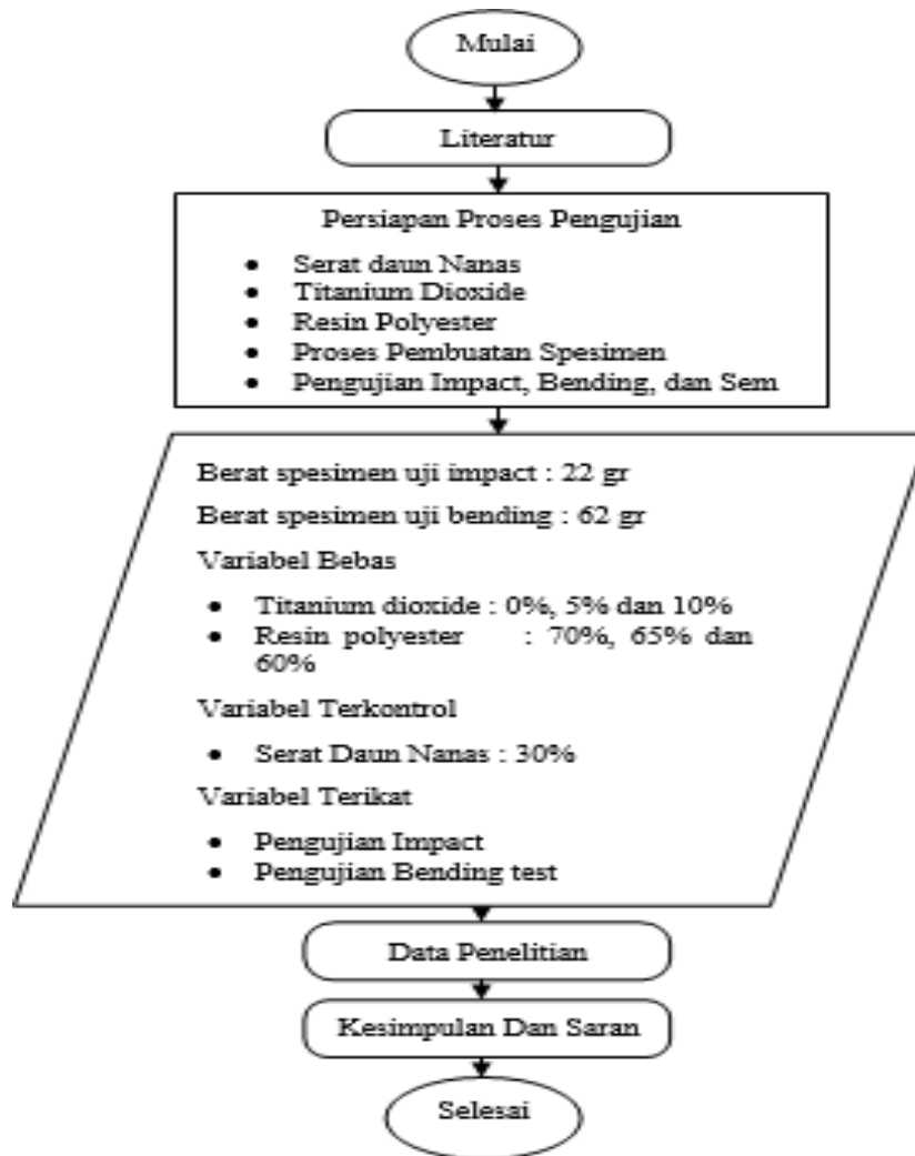
Gambar 1. Diagram Alir
