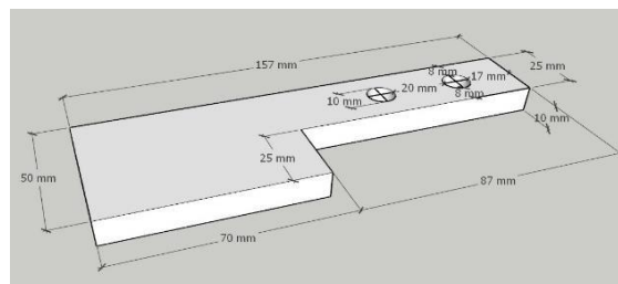
Gambar 7 penahan poros
