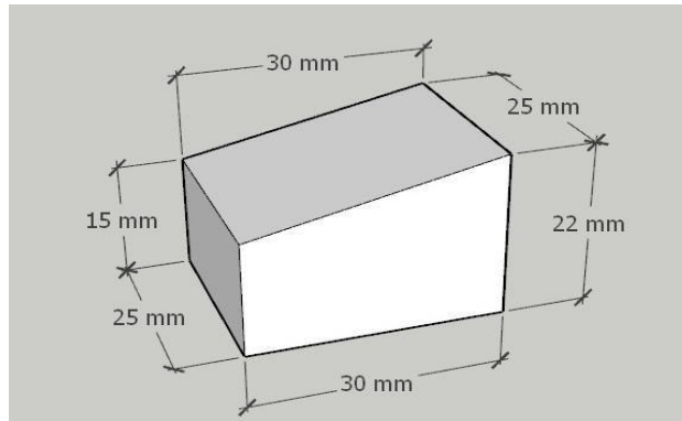
Gambar 4 adjustable jaw
