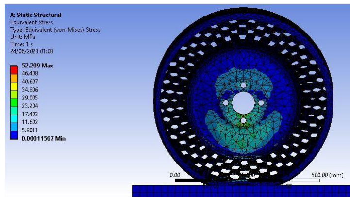
Gambar 11. Nilai distribusi tegangan ban tanpa udara tipe spokes honeycomb
