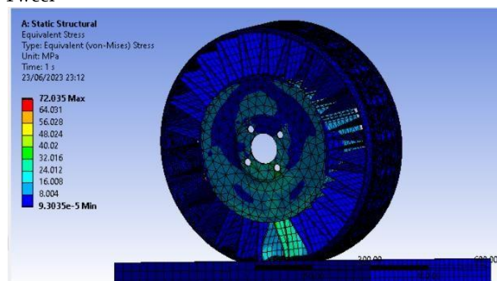
Gambar 10. Nilai distribusi tegangan ban tanpa udara tipe spokes twell
