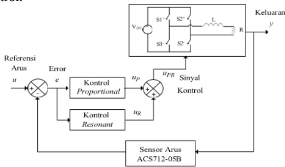
Gambar 10. Diagram Blok Kontrol Propotional Resonant
