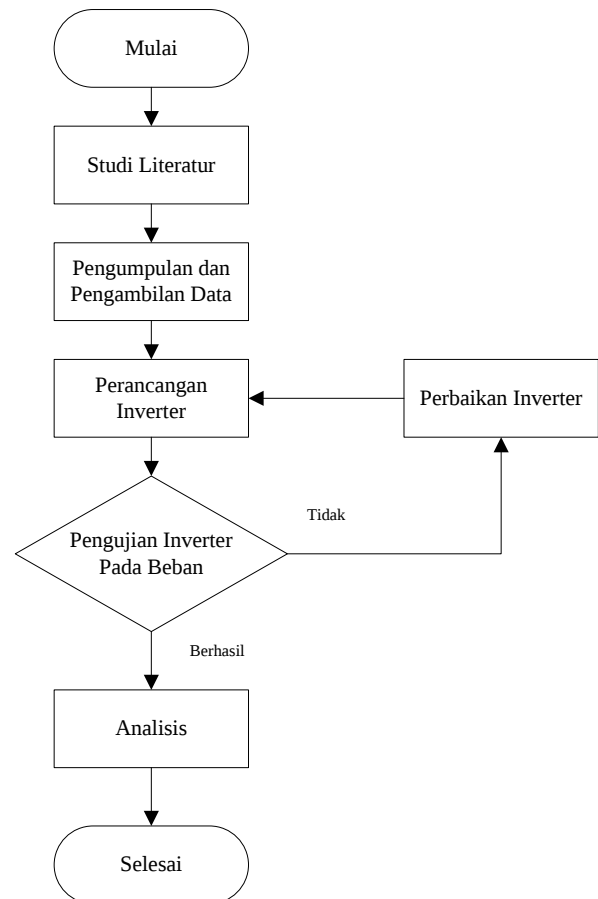
Gambar 12. Flowchart Penelitian
