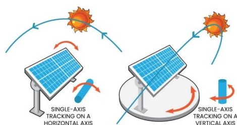
Gambar 2. Panel Surya Tracker Single Axis
