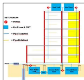
Gambar 10. Distribusi Air down-Feed System Sumber: Google, 2023
