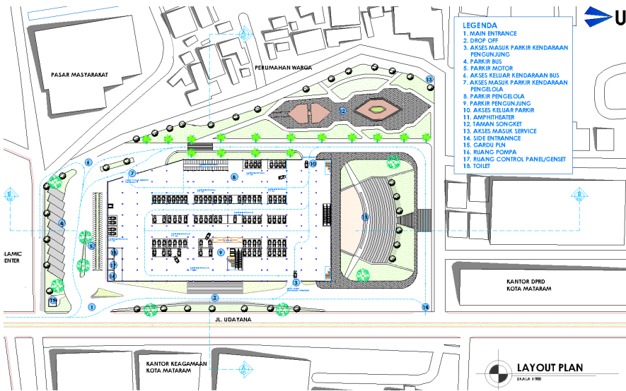
Gambar 11. Layout plan
