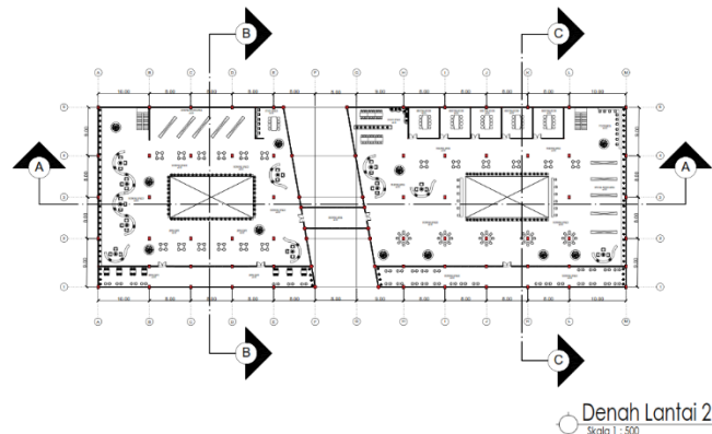
Gambar 11. Denah Lantai 2 Café Library Di Kota Bima
