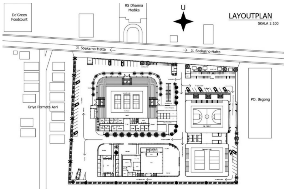
Gambar 17. LayOut Plan
