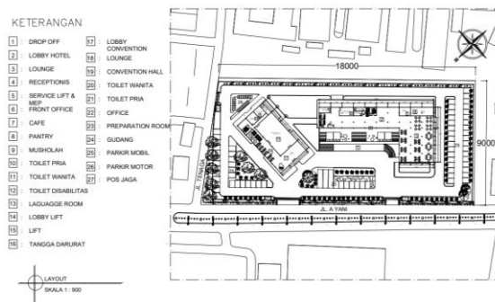
Gambar 13. Layout Plan
