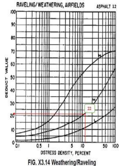
Grafik 2. Nilai Deduct Value Raveling
