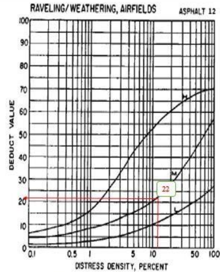
Grafik 2. Nilai Deduct Value Raveling
