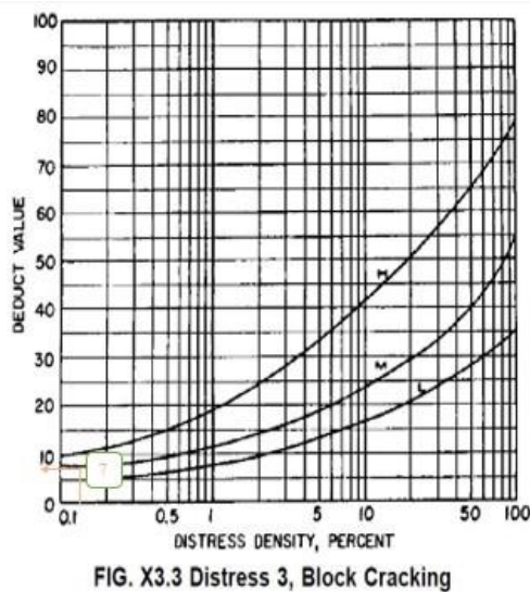
Grafik 7. Nilai Deduct Value Block Cracking
