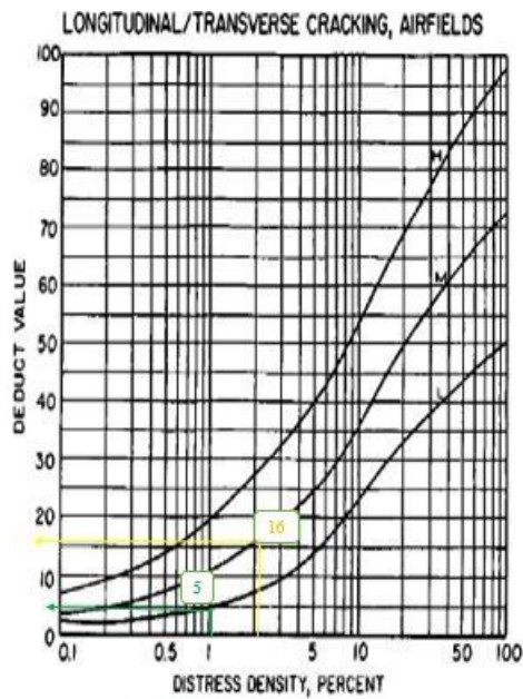
FIG. X3.9 Longitudinal/Transverse Cracking
