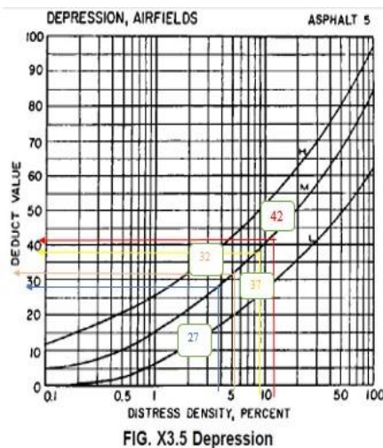
Grafik 1. Nilai Deduct Value Depression
