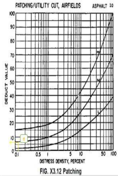
Grafik 5. Nilai Deduct Value Patching
