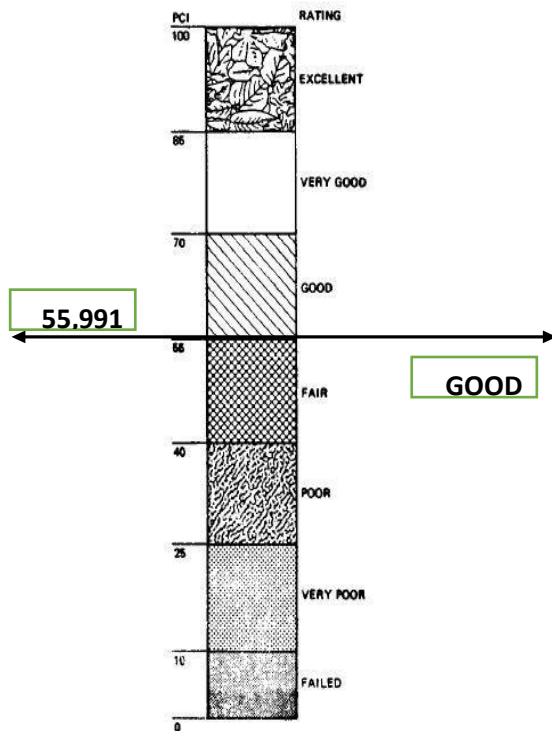
FIG. 1 Pavement Condition Index (PCI) and Rating Scale
