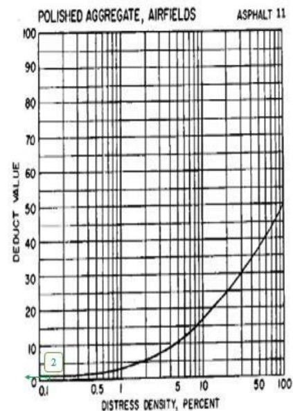
FIG. X3.13 Polished Aggregate
