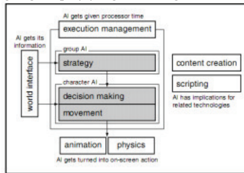
Gambar 1. Model game AI [1]
