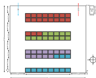
Gambar 3 Desain 2D Layout Usulan
